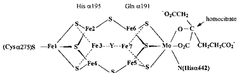
Fig. 5. Proposed FeMo-cofactor structure in nitrogenase MoFe-protein (adapted from Ref. [20]).
