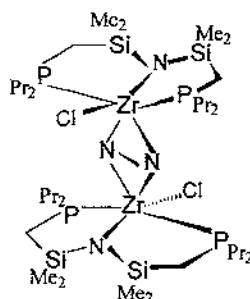
Fig. 23. Molecular structure of the complex \{[(i-Pr_2PCH_2SiMe_2)_2ZrCl]_2\}(\mu-\eta^2:\eta^2-N_2) [129].
