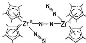
Fig. 19. Structure of the \{[\pi\text{-C}_5(\text{CH}_3)_5]_2\text{Zr}(\text{N}_2)\}_2\text{N}_2 complex.
