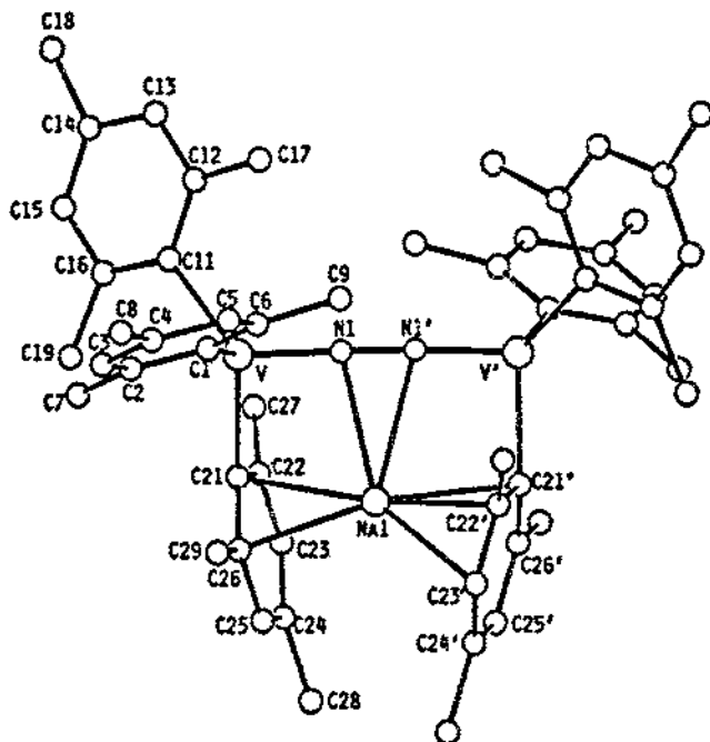
Fig. 22. A view of the anion in the dinitrogenmesitylvanadium complex [119].
