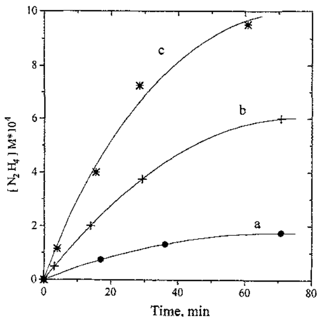
Fig. 16. Kinetics of hydrazine formation in dinitrogen reduction in the presence of three Mo complexes: (a), formed by reduction of complex [\text{Mo}(\text{V})\text{OMg}(\text{MeOH})_2(\text{OMe})_5]_2 (Fig. 12); (b), formed by reduction of complex \{[\text{Mg}_2\text{Mo}_8\text{O}_{22}(\text{OMe})_6(\text{MeOH})_4]^{2-}[\text{Mg}(\text{MeOH})_6]^{2+}\} \cdot 6\text{MeOH} (Fig. 14); (c), acid treatment of complex 3 (Fig. 14).
