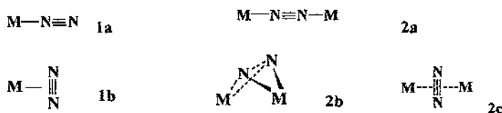
Fig. 3. Modes of dinitrogen bonding.
