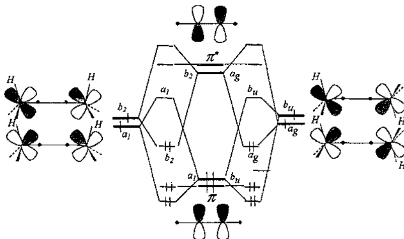
Fig. 18. MO diagram for cisoid and transoid configurations of the complex (Cp_2TiH)_2N_2 .
