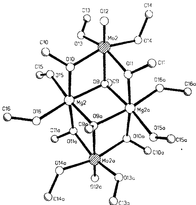
Fig. 12. View of the complex 1 : [\text{Mo}(\text{V})\text{OMg}(\text{MeOH})_2(\text{OMe})_5]_2 .
